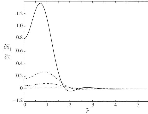
FIGURE 7. Entropy production in the Taylor vortex when Pr = 1 , C_1 = e^{1/2}/2 , \tau_i = \frac{1}{2} .
